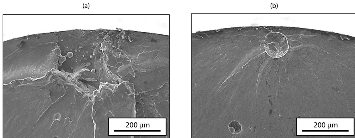
Fig. 8 Fractographic identification of crack initiation side for (a) batch A [SR] at 70 MPa and N_f = 1.6E6 and (b) batch A [SR] at 70 MPa and N_f = 3.2E8 (1)
